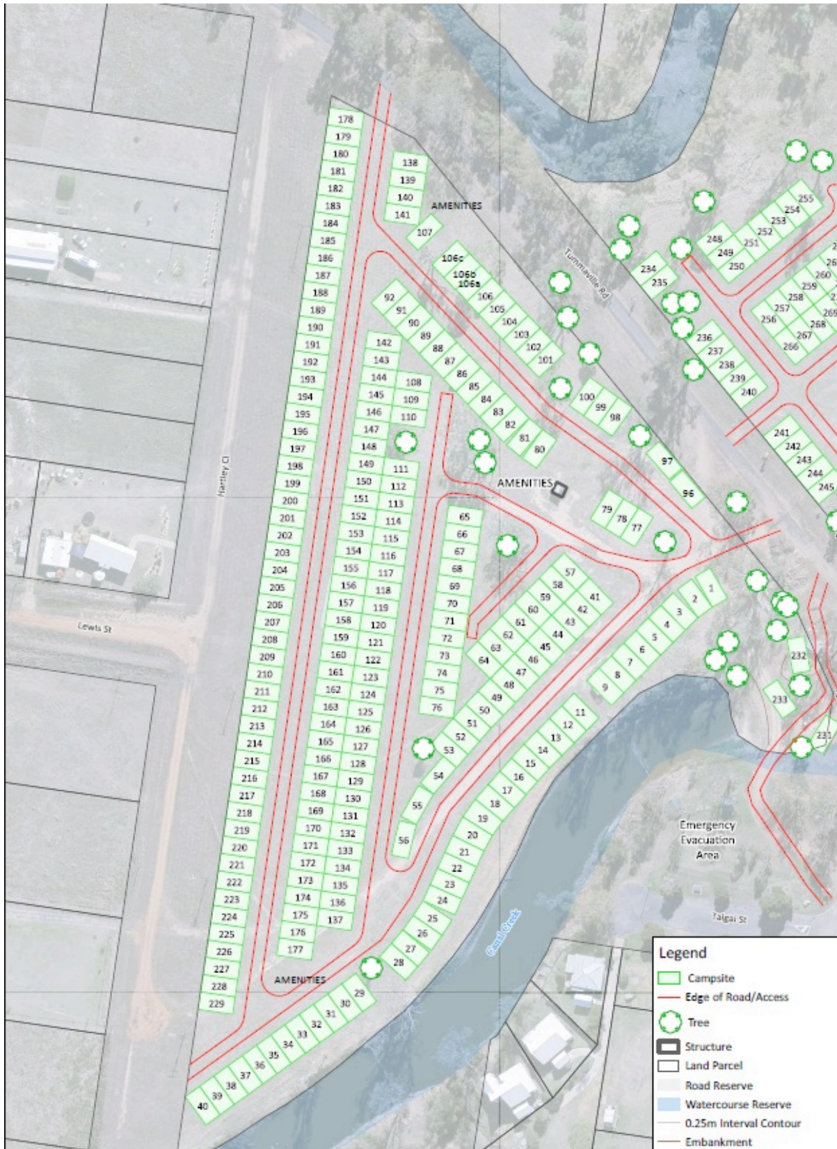
Leyburn Sprints Campground West Layout Date: 20-Mar-2019 By: DTS Drawing: MGA-94 Zone 56
